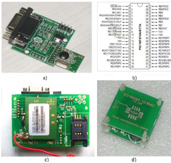
Fig. 2. PIN diagrams of different components used in our prototype. (a) ZigBee module CC2500. (b) Pin diagram of PIC16F877A. (c) GSM Module SIM300. (d) RFID reader-125 kHz-TTL.
